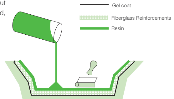
Hand Lay-up
